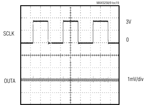
CLOCK FEEDTHROUGH
